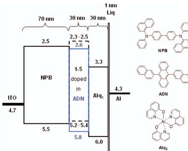
Figure 2. Relative energy-level alignments and layer thickness of OLEDs.
