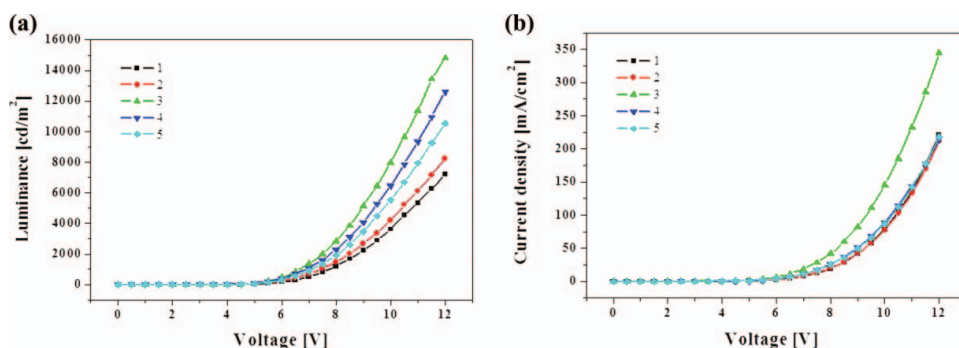
Figure 5. (a) Luminance and (b) current density versus applied electric voltage characteristics of devices 1–5 .
