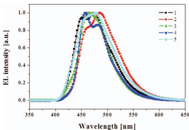
Figure 3. EL spectra of devices using the five stilbene derivatives as dopant emitters.
